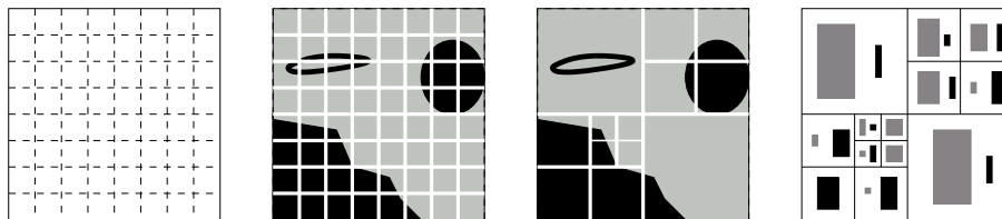
Figure 5.2. A useful set of events \mathcal{T} for images which would focus on pixel localization can be represented by a grid, such as the 8 \times 8 one represented above. In this case P_3 corresponds to the 4^3 windows presented in the left image, P_2 to the 16 larger square obtained when grouping 4 small windows, P_1 to the image divided into 4 equal square parts and P_0 is simply the whole image. Any partition of the image obtained from sets in P_0^3 , such as the one represented above, can in turn be used to represent an image as a family of sub-probability measures, which reduces in the case of two-color images to binary histograms as illustrated in the right-most image.
