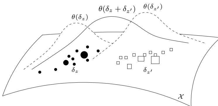
Figure 3.1. Measure representations of two lists z and z' . Each element of z (resp. z' ) list is represented by a black circle (resp. a white square), the size of which represents the associated weight. Five measures of interest are represented: the image measures \delta_z and \delta_{z'} of those weighted finite lists, the smoothed density estimates \theta(\delta_z) and \theta(\delta_{z'}) of the two lists of points, and the smoothed density estimate \theta(\delta_z + \delta_{z'}) of the union of both lists.
