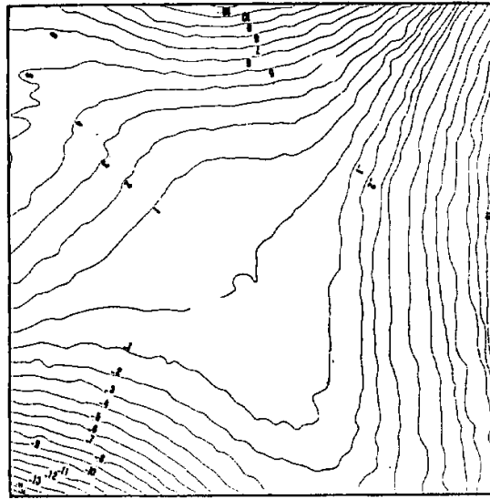
Figure 3 Realization of a 2-IRF with the GC K(h) = -|h|^5 . The representation chosen, as well as its first and second derivatives, vanishes at the center of the figure (from Orfeuil [10]).
